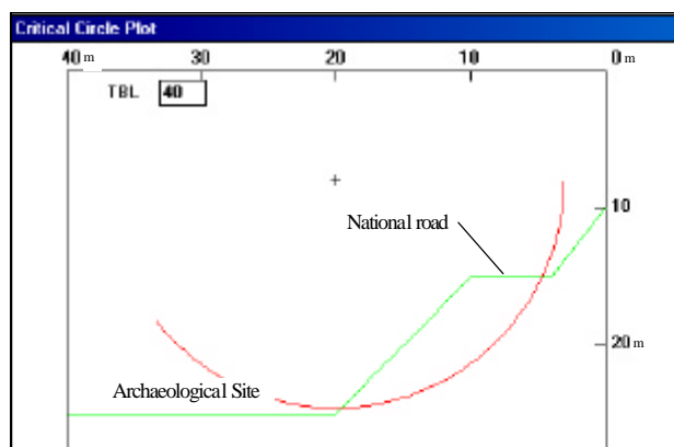
Figure 6. Stability analysis ( SF=0.17 ) of the lower part of the slope (under the road), located at the north end of the archaeological site of Olympia.
