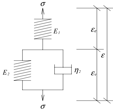
Figure 1. Three-element visco-elastic model
