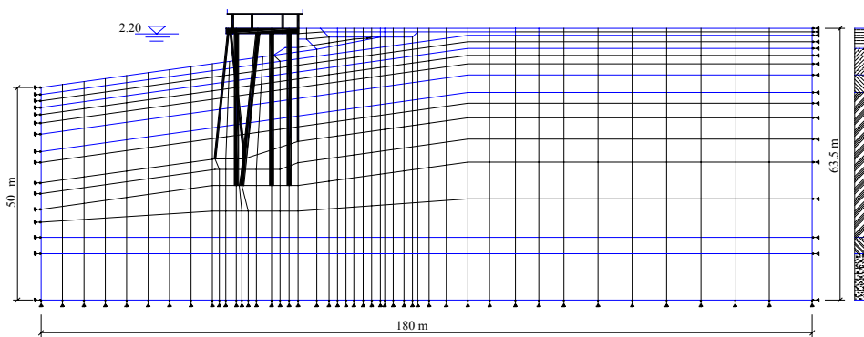
Figure 3. FEM mesh for settlement analysis of flood-control wall
