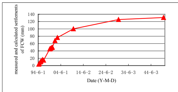
Figure 4. Increase of calculated structural settlement of FCW with time
