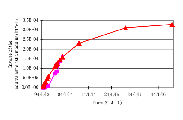
Figure 5. Relationship between equivalent elastic modulus and time
