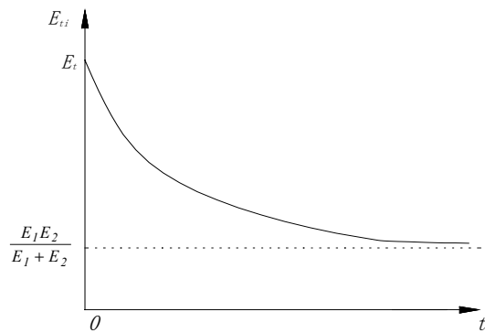
Figure 2. Relationship between equivalent elastic modulus and time of three-element visco-elastic model
