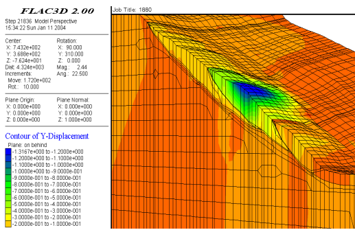
Figure 4. Contour map of vertical displacement
