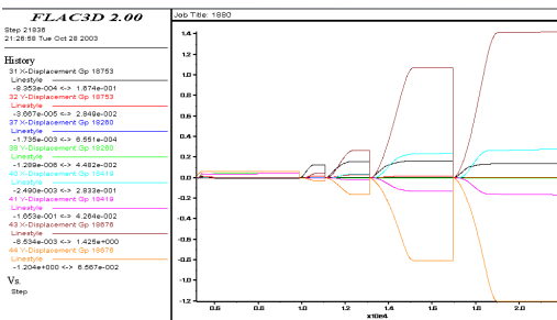
Figure 5. Displacement Histories at Some Points in the Slope
