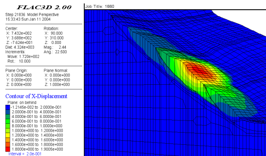
Figure 3. Contour map of horizontal displacement
