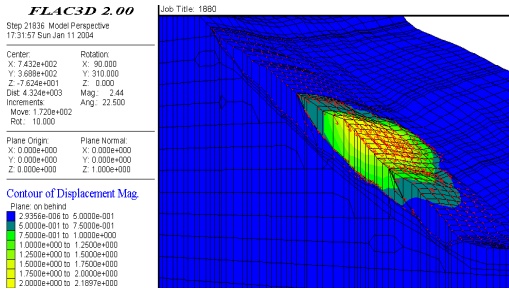
Figure 2. Contour map of U-Displacement
