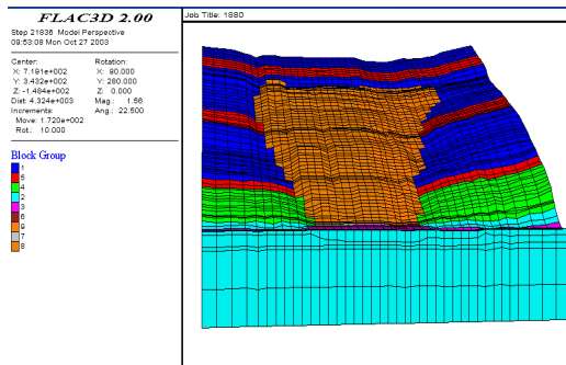
Figure 1. 3D numerical model
