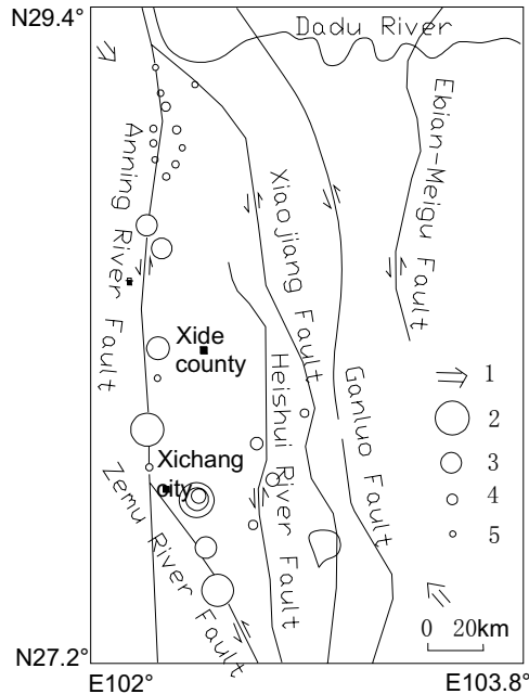
Figure 1. Seismic-tectonic map of Xichang (from Yue-Quan Shang, 1992) 1. \sigma_1 , 2. seismicity >7 , 3. seismicity =6\sim6.9 , 4. seismicity =5\sim5.9 , 5 seismicity <5
