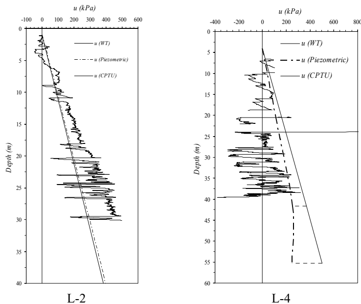
Figure 5. Pore pressure profile for: L-2 (a) and L-4 (b) sites
