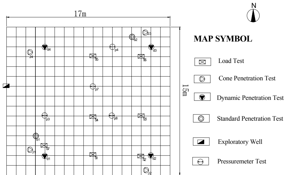
Figure 3. Layout of the YY1 site
