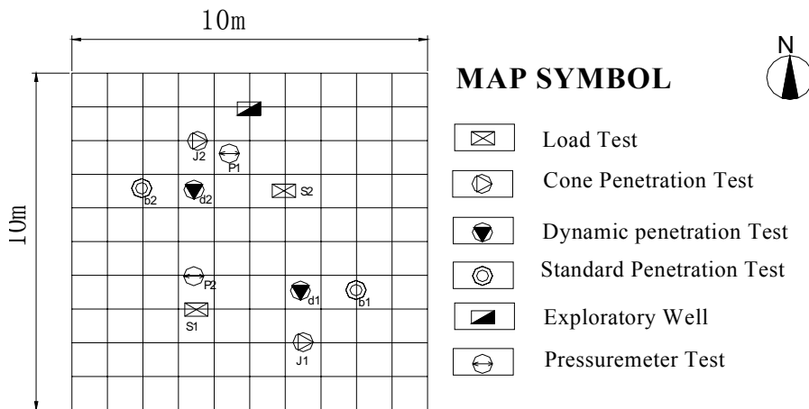
Figure 4. Layout of the YY2 site
