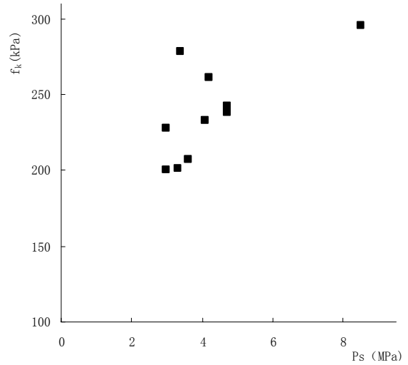
Figure 6. Relationship between the bearing capacity of deep soil layer ( f_k ) and CPT ( P_s )
