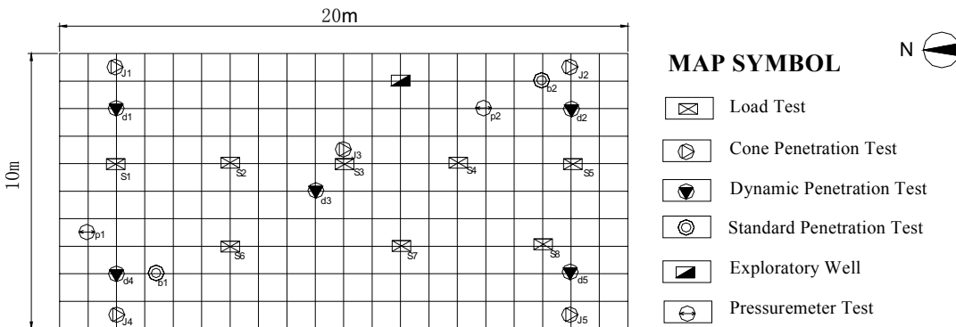
Figure 2. Layout of the DY site
