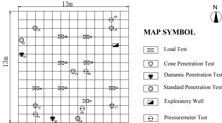
Figure 1. Layout of the CL site
