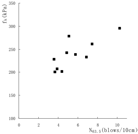
Figure 5. Relationship between the bearing capacity of deep soil layer ( f_k ) and DPT ( N_{63.5} )
