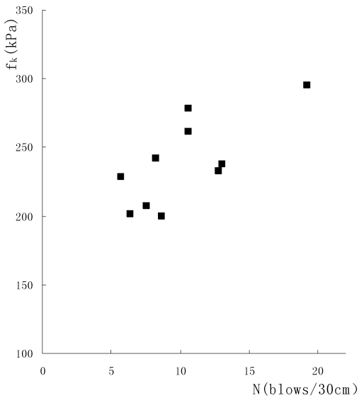
Figure 7. Relationship between the bearing capacity of deep soil layer ( f_k ) and SPT ( N )
