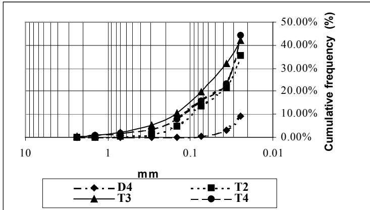
Figure 1. Particle size distribution of residual sludges from gang saw (Ossola Valley Basin and Luserna Stone Basin). D4: sludge from diamond frame-saw (LSB); T2: sludge from the gang saw (LSB); T3 and T4: the gang saw (VCO).
