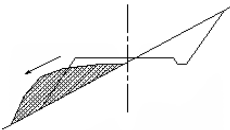
Figure 3. The slippage of dug and filled roadbed by the action of deadweight and water
