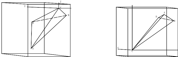
c. Double-slide formed by I and II structural plane d. Single-slide formed by structural plane I and II
