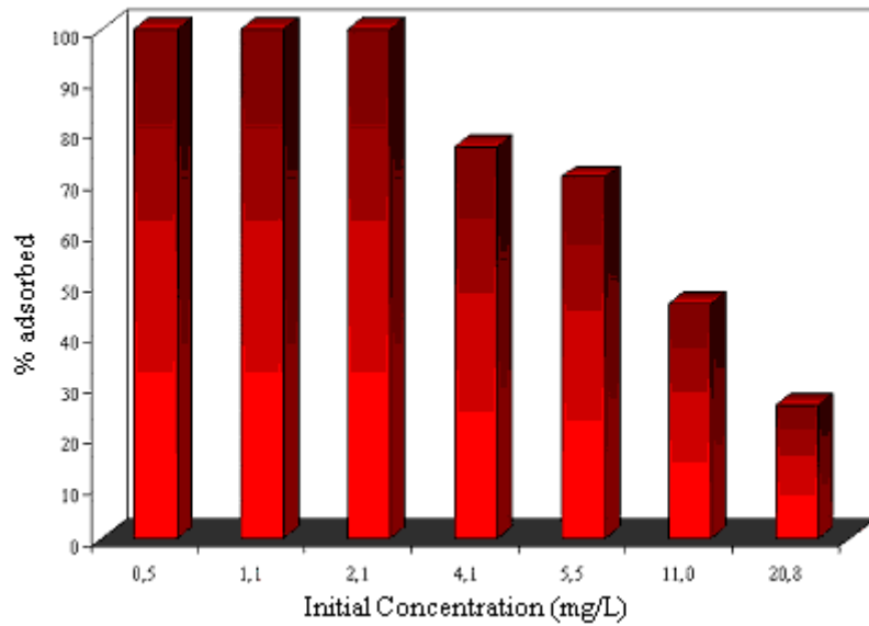
Figure 3. Percentage of Pb adsorbed in the soil as function of the initial concentration.
