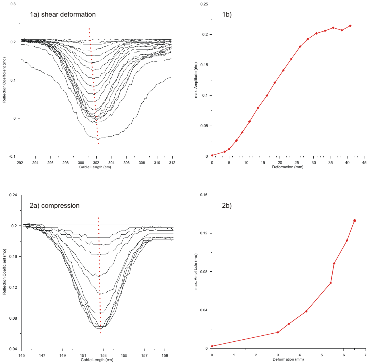
Figure 3. Comparison of TDR measurement results when shearing (1) and compressing (2) the coaxial cable. Note the progressive displacement of the peak maximum (shown by the red dotted line) with proceeding deformation when the cable is sheared (1a), whereas it stays more or less static when the coaxial cable is compressed (2a). This suggests a likely method for distinguishing the deformation mechanism. The increase of maximum amplitude with progressive deformation is shown in diagrams 1b and 2b for shear deformation and compression, respectively. Measurements were made with a Campbell Scientific TDR 100 Time Domain Reflectometer and a CommScope P3 500 CA coaxial cable of 12 mm diameter.
