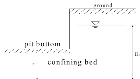
Figure 2. Figure for pit bottom sudden surge checking calculation
