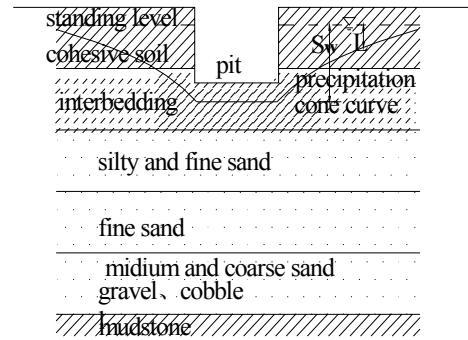
Figure 3. Figure of water level as lowering the confined water
