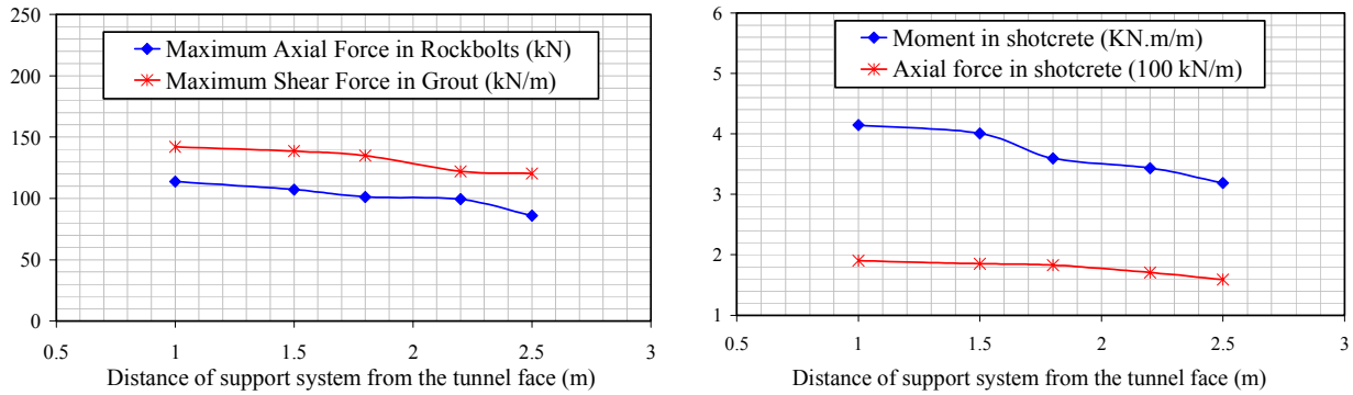
Figure 10. Effect of distance of support system from the tunnel face on rockbolt and shotcrete forces
