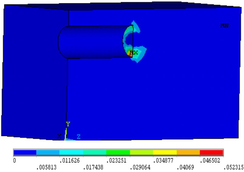
Figure 4. Plastic deformation at \sigma_1 = 75.66 kPa
