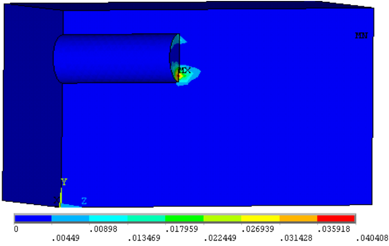
Figure 3. Plastic deformation at \sigma_1 = 70 kPa
