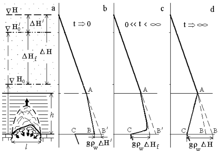
Figure 1. Mechanism of hydraulic fracturing (a), and pore pressure diagrams at the initial moment (b), intermediate stage of downward seepage (c) and final one (d). \nabla H : water-table (the level of unconfined water); \nabla H'_0 and \nabla H_0 : potentiometric level of karst water before and after water head decline; l : the span of a cavern (rock void) at the base of karst overburden; h : the thickness of confining bed; t : time. Big arrow and small ones show respectively the propagation of crumbling front and the "shooting" of clay spalls and pieces from the roof of soil void.
