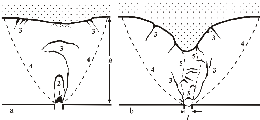
Figure 5. Modeling failure of the Upper Permian clay bed ( h/l = 13,5 ) in an area of Dzerzhinsk city (Russia) at the initial-middle (a) and final (b) stages of hydraulic fracturing; 1: soil cavity; 2: zone of clay extrusion; 3: breakdown fractures; 4 and 5: boundaries of visible deformation and open hole, respectively.
