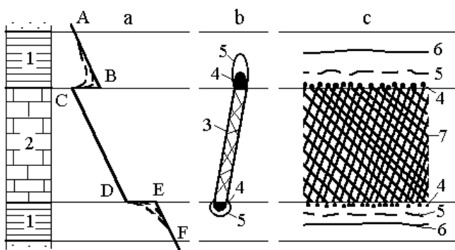
Figure 6. Conceptual model of weak interbed formation (c) under water head reduction (a); 1: confining bed and aquitard; 2: confined aquifer; 3: a single fissure; 4: soil voids; 5: zones of crumbling and extrusion; 6: boundaries of weak interbeds; 7: fissure system; ABCDEF: fluid pressure diagram.
