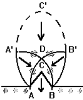
Figure 2. Region of influence of opening AB in the rigid base of a soil mass. ACB: falling block or cave-in zone; ADB: relieved arch or zone of dilatancy and potential cave-in; AA'D and BB'D: plastic wedges or zone of bearing pressure and potential slippage; DA'C B: zone of transit from anomalously high and low stresses to geostatic ones (zone of possible extrusion of fissured solid by downward water flow). Big arrows and small ones show the directions of potential soil flow and those of maximal tangential stresses.
