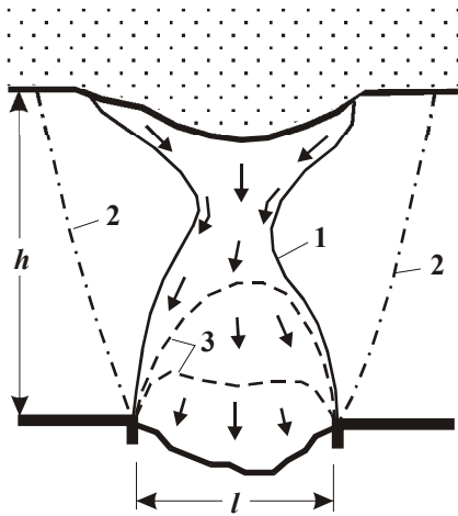
Figure 4. Extrusion zone (1) in the Upper Carboniferous and Upper Jurassic clays joined in a single stratum ( h/l = 1,6 ) in the area of Tukhachevsky street in Moscow city (the results of physical model tests); 2 and 3: boundaries of open hole and soil cavity at the final and initial stages of fracturing, respectively. Arrows show the flow direction of crumbled clay solid.
