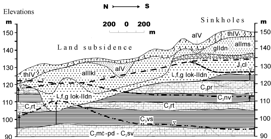
Figure 7. Hydrogeological cross-section through the rock massif; thIV, alV: the Holocene anthropogenic deposits and alluvial sediments of the flood land; aIIkl: the Upper Pleistocene alluvial sediments of the second stream terrace; aII, gII: the Middle Pleistocene alluvial sand of the third terrace and glacial clay loam; l,f,gI-II: the Lower-Middle Pleistocene fluvio-glacial sand and limnoglacial loamy sand; J_3cl : the Upper Jurassic clays; C_3pr , C_3rt , C_3nv , C_3vs : the Upper Carboniferous carbonate rocks of the Perkhurovskaya and Ratmirovskaya Formations and clay rocks of the Neverovskaya and Voskresenskaya Formations; C_2mc-C_3sv : of the Upper and Middle Carboniferous limestones and dolomites; dotted lines and arrows show water table and piezometric levels. piezometric
