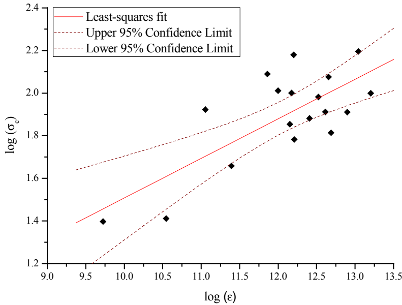
Figure 5. Relationship between logarithm of both uniaxial compressive ( \log(\sigma_c) ) strength and waveform energy ( \log(\epsilon) ).
