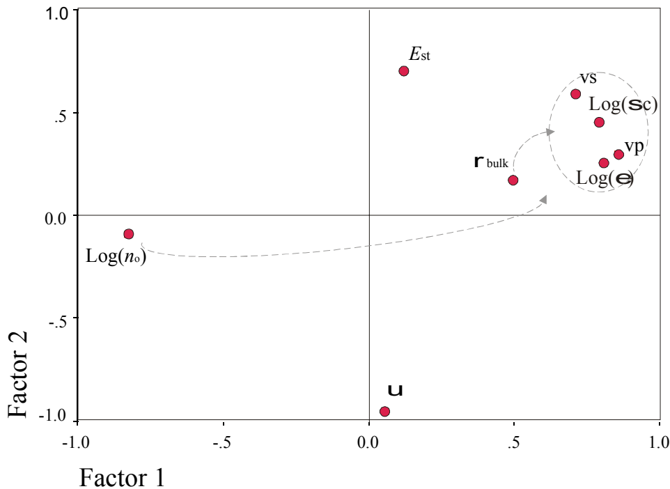
Figure 2. Principal component analysis with the most representative variables: P-wave velocity ( v_p ), S-wave velocity ( v_s ), waveform energy logarithm ( \log(\epsilon) ), density ( \rho_{\text{bulk}} ), effective porosity logarithm ( \log(n_o) ), compressive strength logarithm ( \log(\sigma_c) ), Young static elasticity modulus ( E_s ) and Poisson's ratio ( \nu ).
