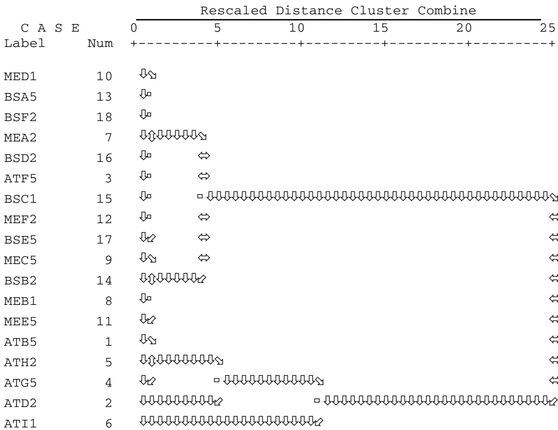
Figure 7. Cluster Analysis of the samples as a function of its mechanic properties (AT: Amarillo Triana; BS: Beige Serpiente; ME: Marrón Emperador).
