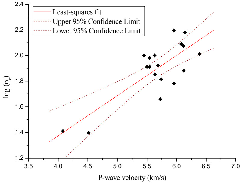
Figure 3. Relationship between logarithm of uniaxial compressive strength ( \log(\sigma_c) ) and P-wave velocity.
