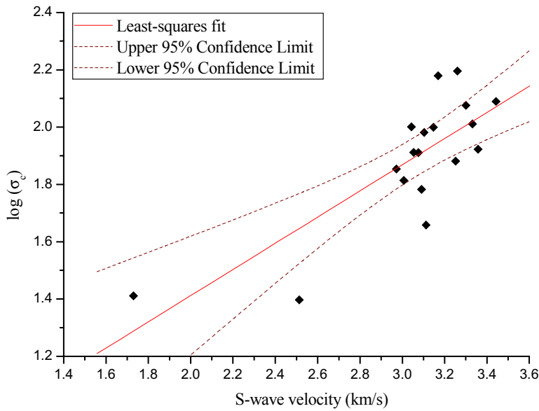
Figure 4. Relationship between logarithm of uniaxial compressive strength ( \log(\sigma_c) ) and S-wave velocity.
