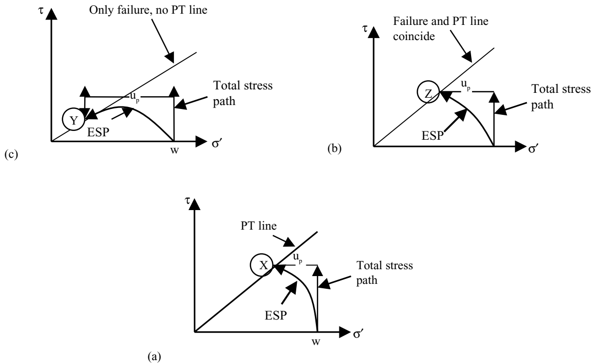
Figure 2. Schematic diagrams illustrating the concepts of least dilation and critical pore pressure (a) dilation (b) critical (c) liquefaction
