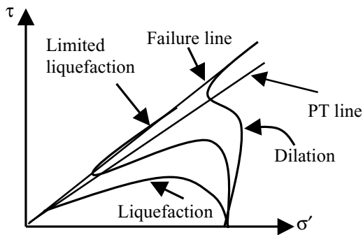
Figure 1. A sketch of the three basic behaviors of granular materials (after Castro 1969)
