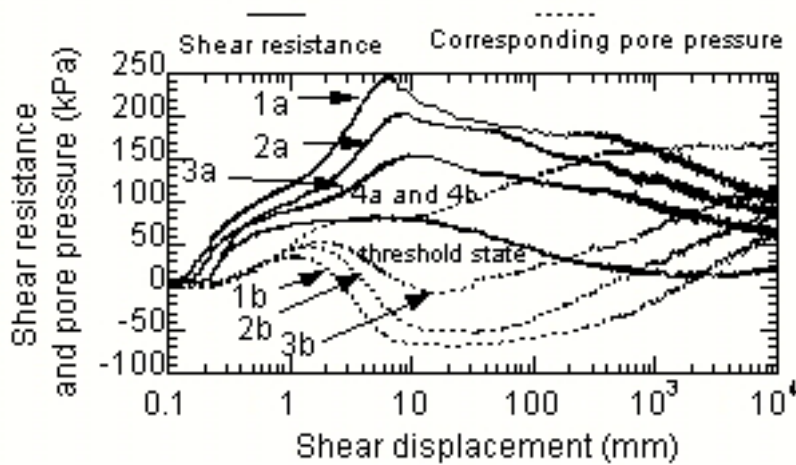
Figure 8. Shear resistances and the corresponding pore pressures of some sands as density changes (specimens at 196kPa confining stress)
