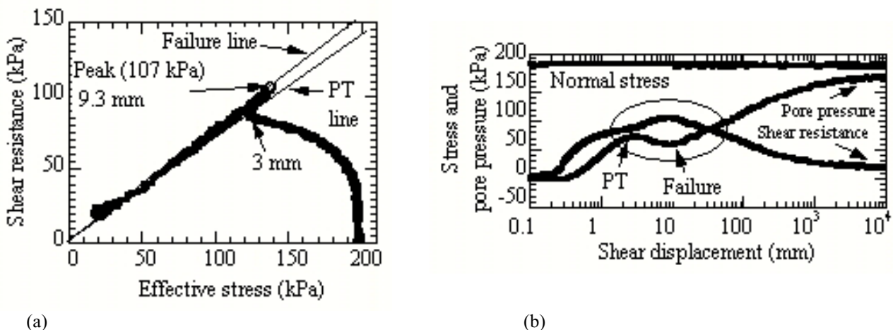
Figure 7. (a) Typical stress path showing significant dilation because pore pressure and shear resistance at PT are not equal (b) Stress versus shear displacement
