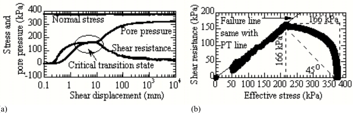
Figure 5. (a) Pore pressure and shear resistance behavior of Takarazuka (b) Stress path defining a critical condition
