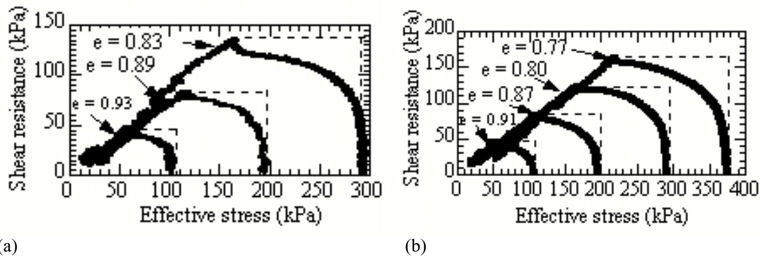
Figure 6. (a) Critical stress paths of silica sands (b) critical stress paths of the Takarazuka landslide sandy specimens
