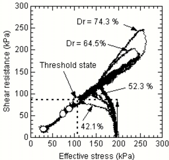
Figure 9. Stress paths illustrating the influence of density on the behavior of silica sand materials
