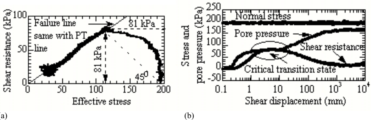
Figure 4. (a) Stress path defining a critical condition (b) Pore pressure and shear resistance behavior of silica sands
