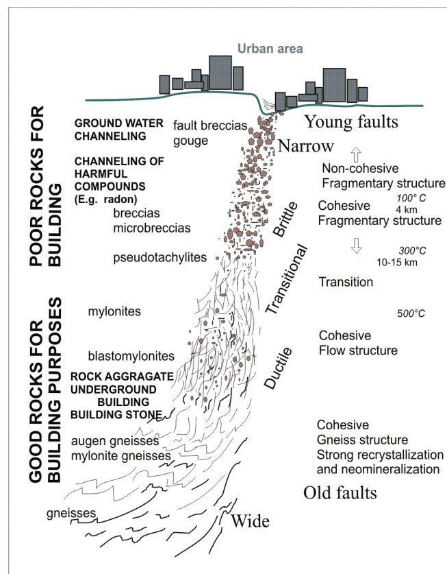
Figure 3. Fault profile with geological fault rock terminology and rock applicability. Our today bedrock surface has imprints of faults formed since Svecofennian times, so they represent different crustal levels
