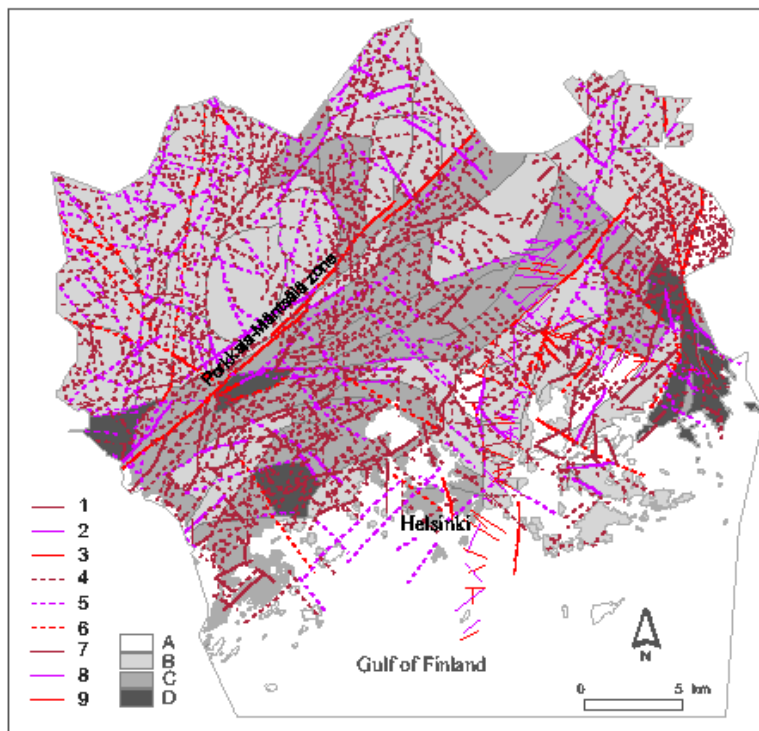
Figure 4. Classified zones of weakness (1-3 observed properties; 4-5 interpreted; 7-9 tunnel data; colours refer for the degree of brokenness, brown is the most intact) and jointing properties (from A to D brokenness increases)
