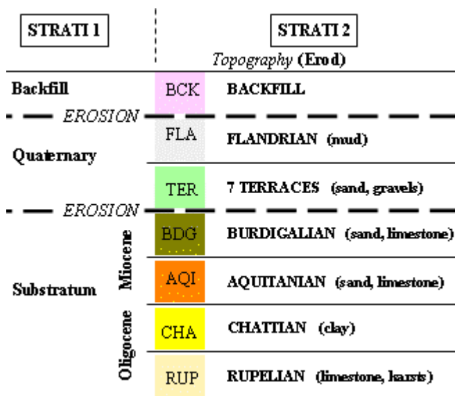
Figure 2. Stratigraphic referential
