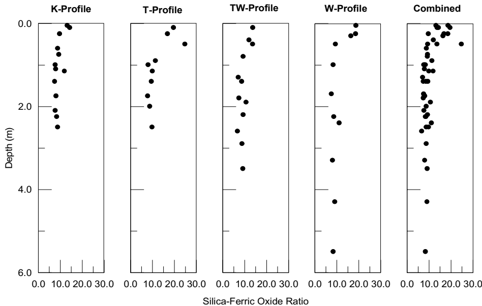
Figure 2. Variations in silica-ferric oxide ratio with depth/degree of weathering at four locations in the Lham Nah Creek Basin
